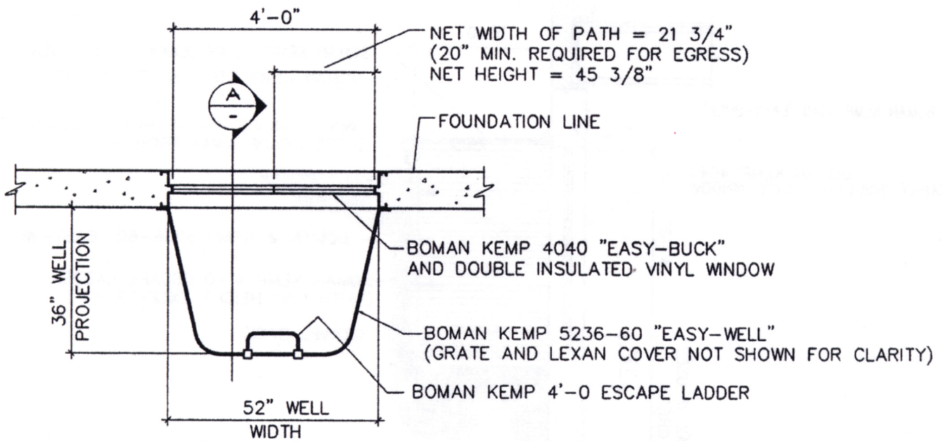
PLAN VIEW WINDOW WELL 36" PROJECTION REQUIRED FOR EGRESS
