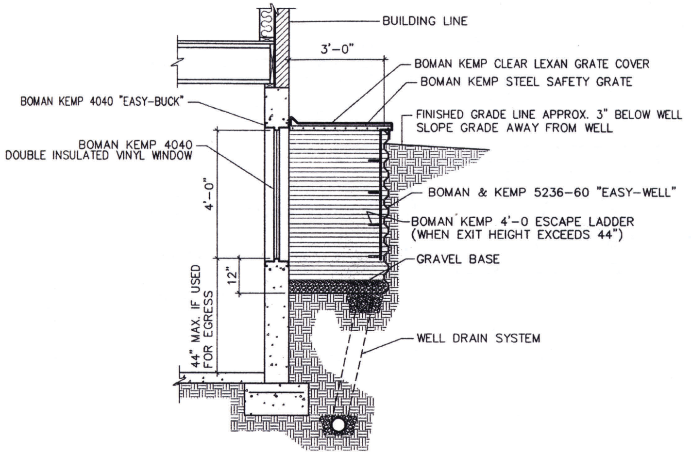
(A) WALL SECTION THRU. WINDOW WELL
